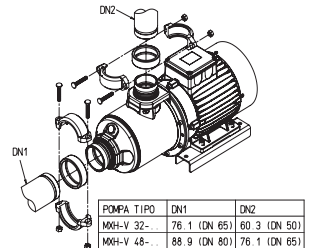
Fig. 8 Bocche con giunti Victaulic Victaulic ports Victaulic-Anschlüsse Raccords Victaulic Acoplamiento Victaulic 进出口卡箍
