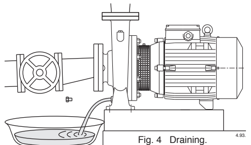
Fig. 4 Draining.
