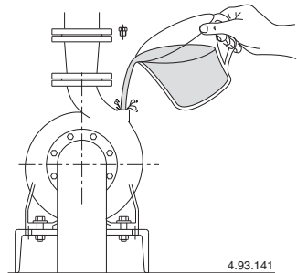
Fig. 3 Filling.
