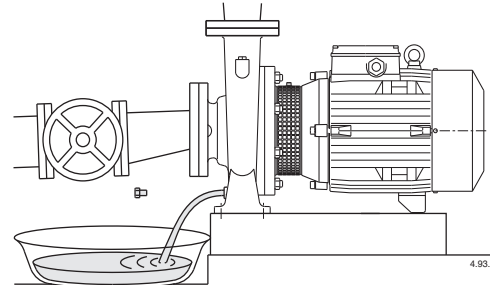
Fig. 4 Draining.
