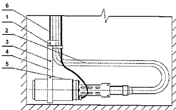
Minimum well clearance 800 mm
