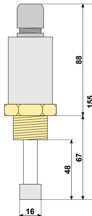
Sonda TVS
